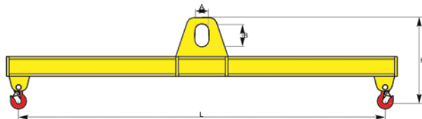
Lifting beam
